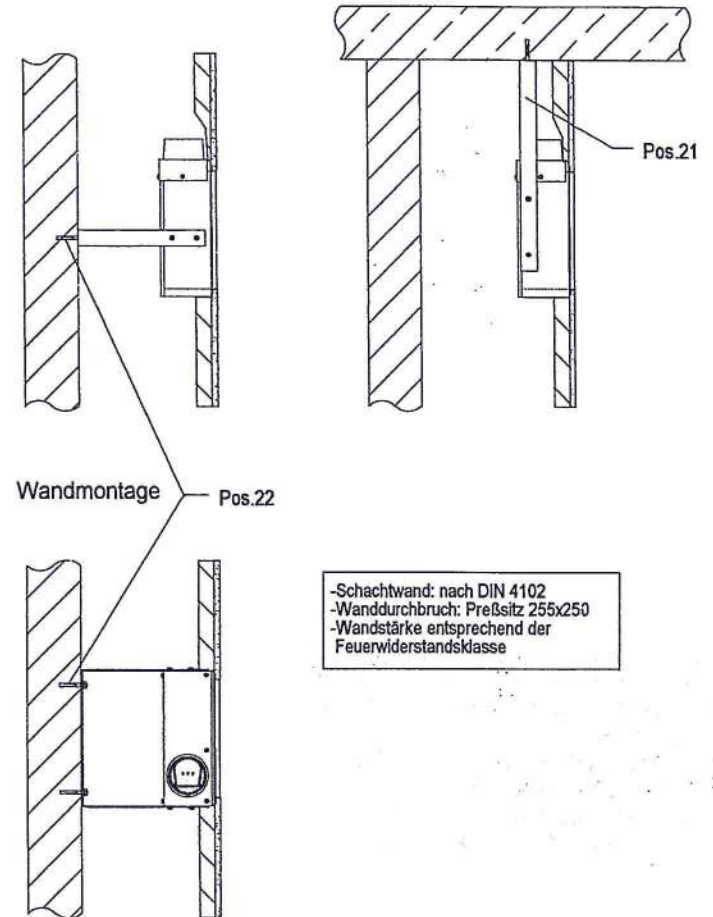
Wandmontage
